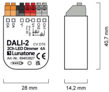
dimensions back box 4A Version 4A Art.Nr.: 89453827
