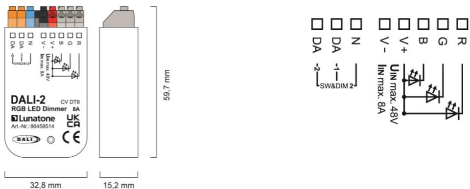
dimensions back box Version 8A Art.Nr.: 86458514 Version 4A Art.Nr.: 89453837
